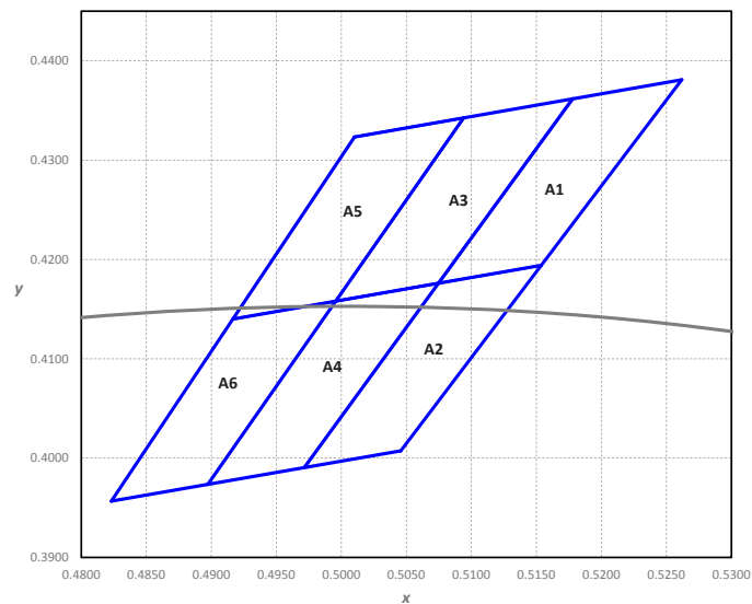
Figure 7: Color bin structure for LUXEON 3535L 2200K.
